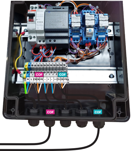
Control box
