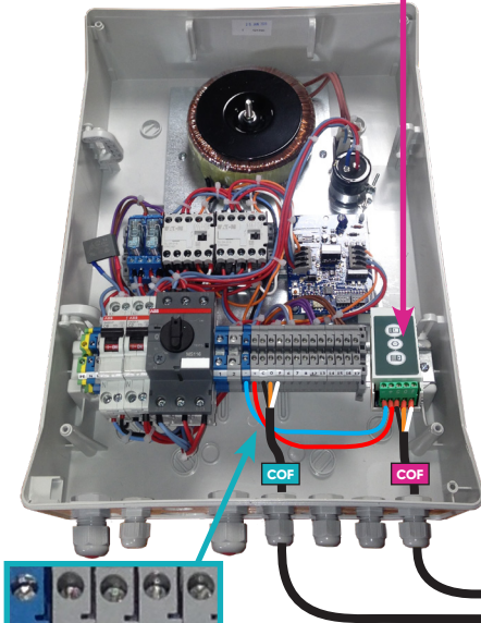
Electrical panel
