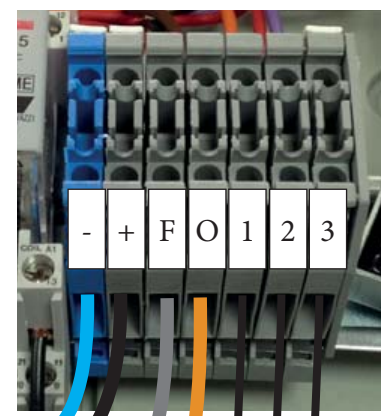
Option Coffret STOP SEL
